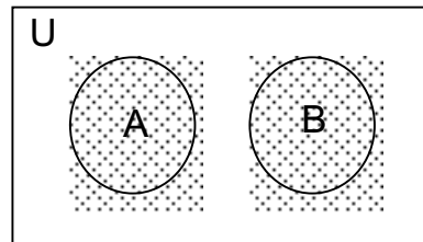
A \cap B = \phi
